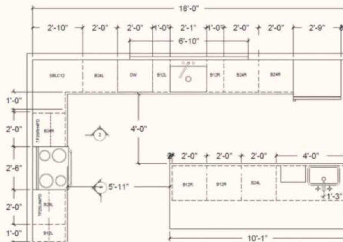
Kitchen Floor Plan - AutoCad
