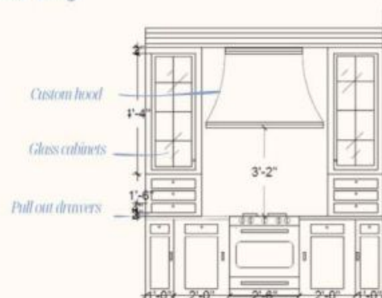
West Wall Elevation - AutoCad
