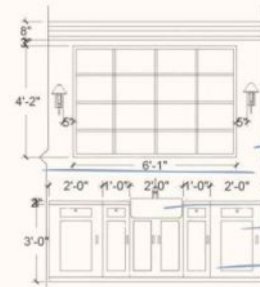
North Wall Elevation - AutoCad
