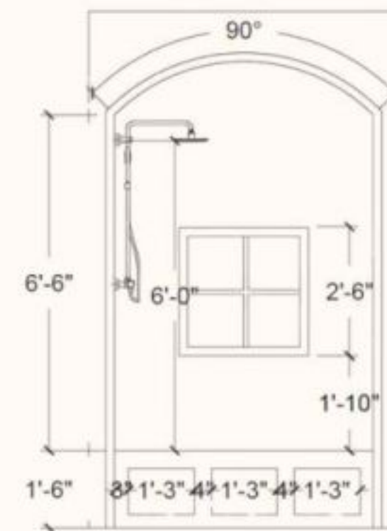
North Wall Elevation - AutoCad
