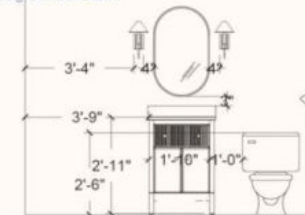
West Wall Elevation - AutoCad
