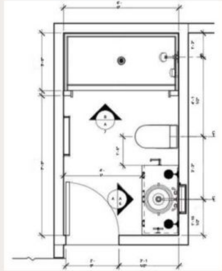
BATHROOM PLAN
