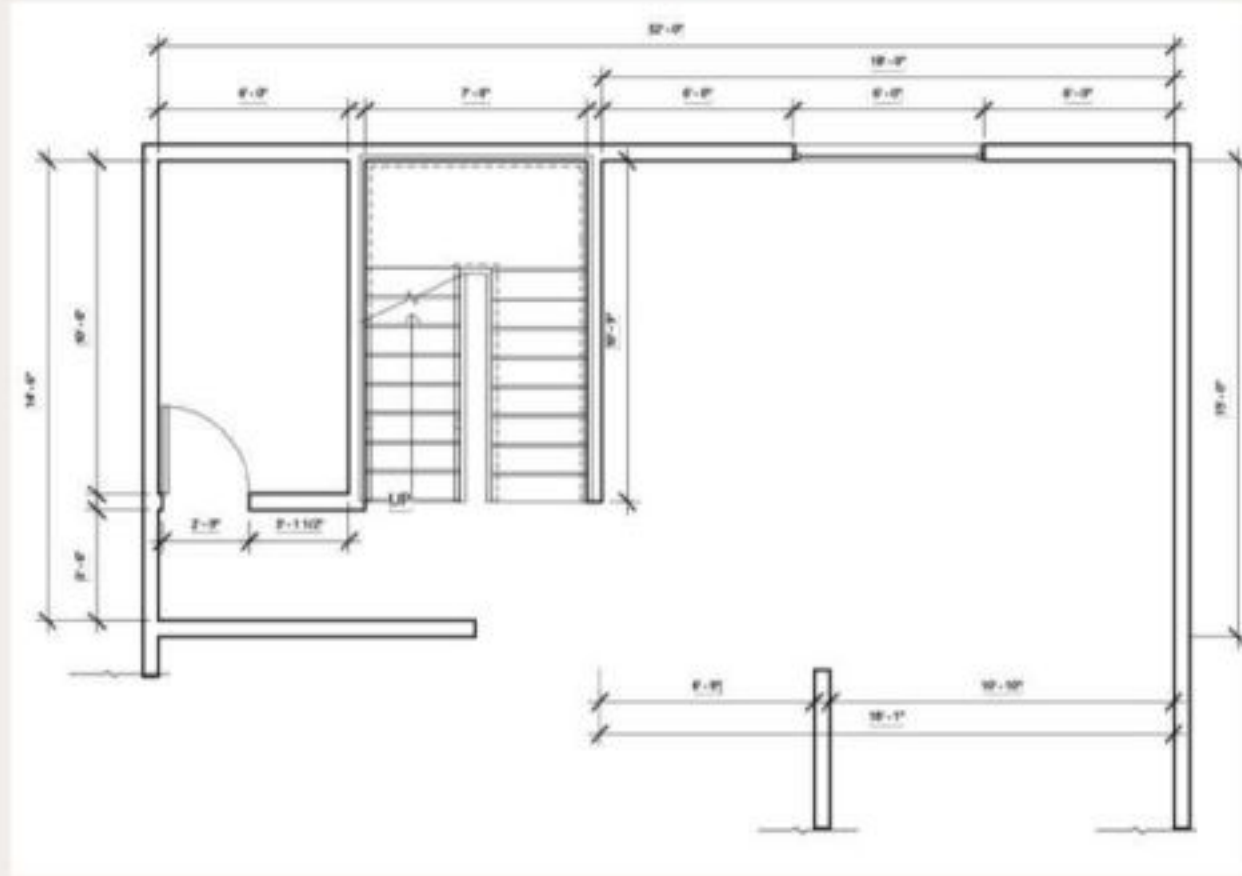
AS-BUILT
