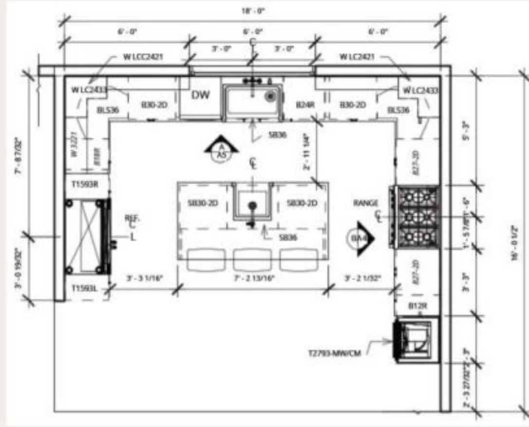
KITCHEN PLAN
