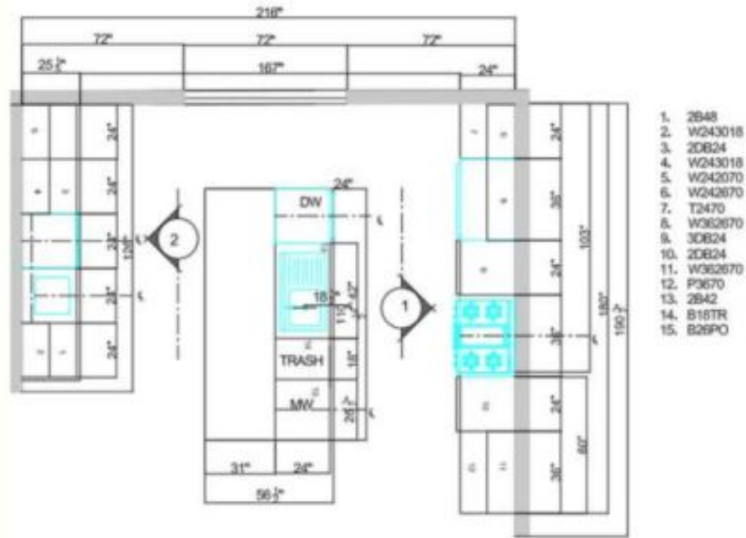
Kitchen Floor Plan AutoCAD
