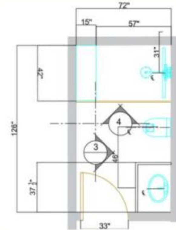
Bathroom Floor Plan AutoCAD
