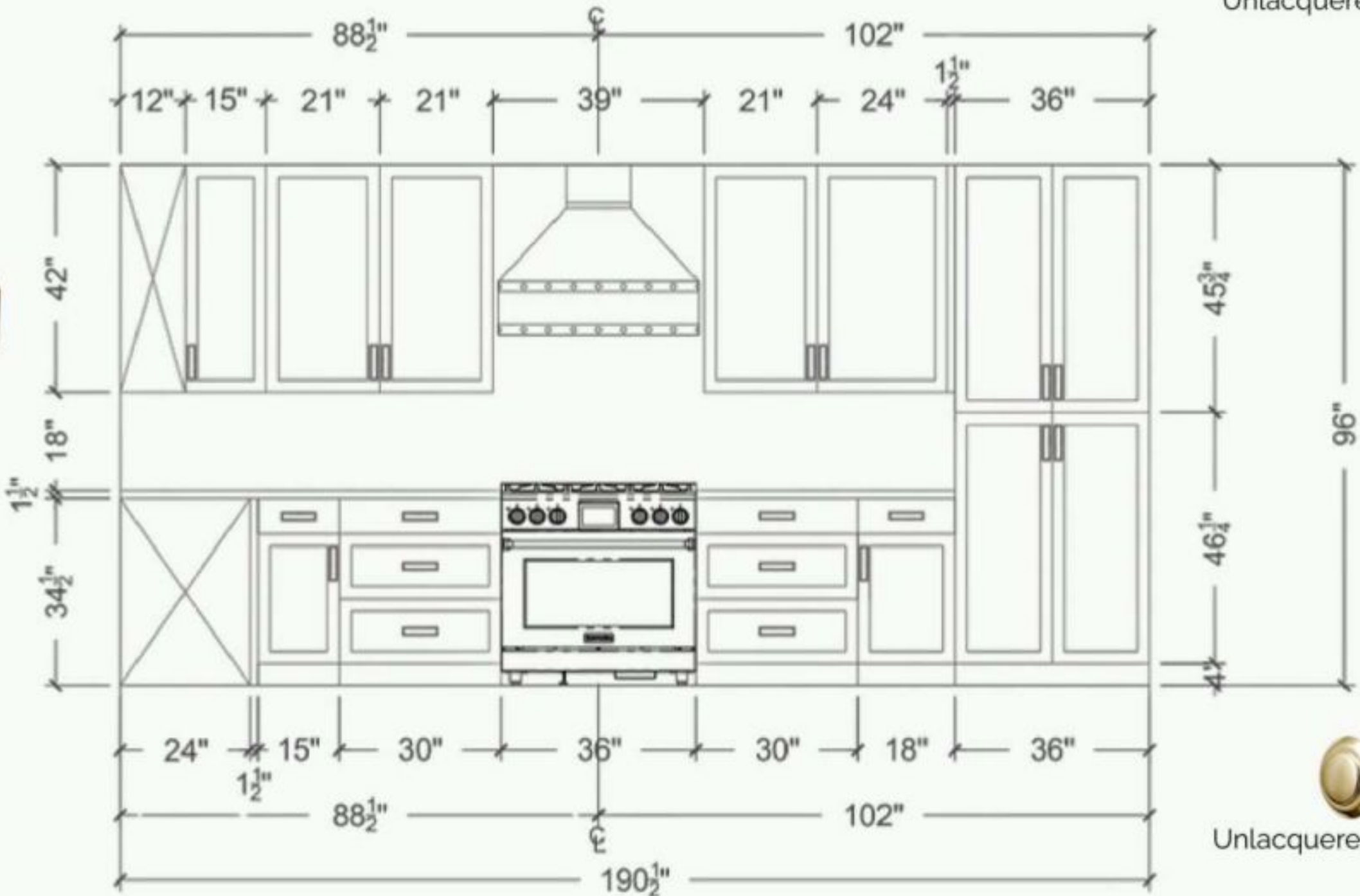
EAST WALL ELEVATION
